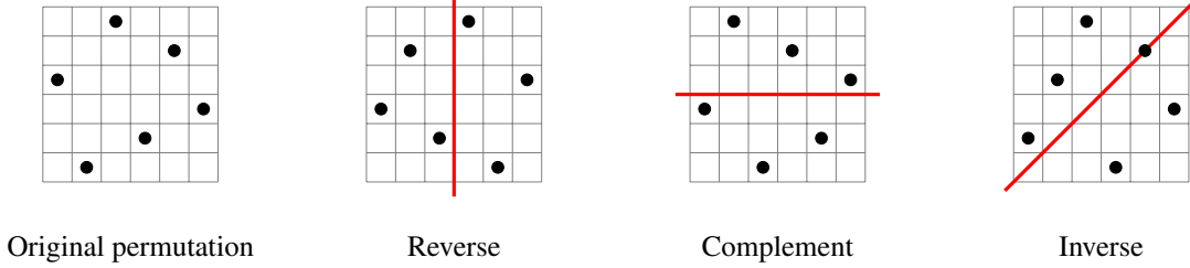
Fig. 1: The diagram of permutation \sigma = 416253 , and its symmetries under r , c and i .
